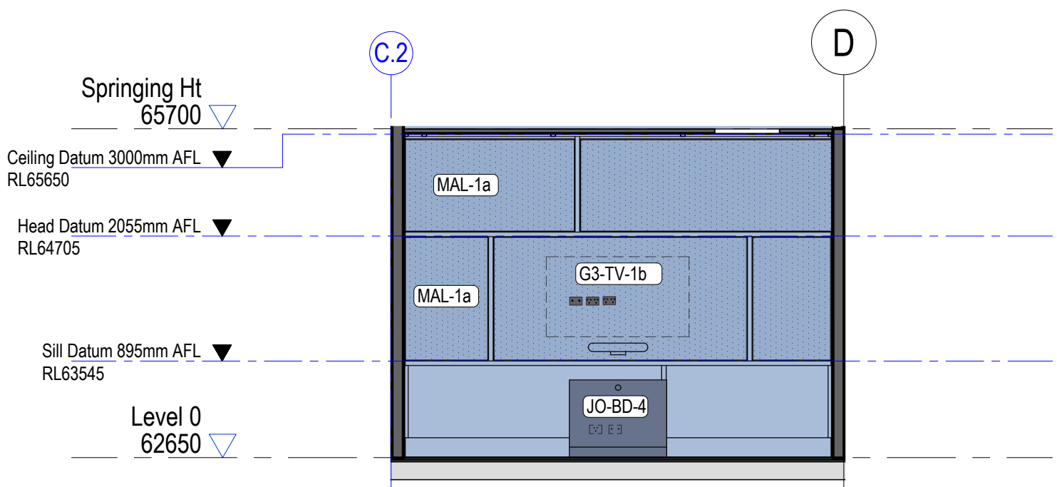
7 0.30 - Meeting 3 - North Elevation 1 : 50
