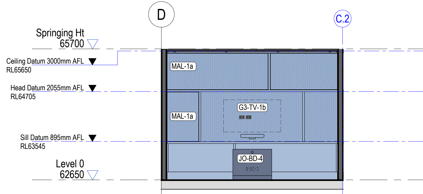
4 0.31 - Meeting 4 - South Elevation 1 : 50
