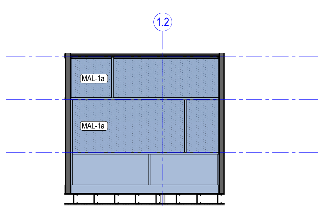
3 0.31 - Meeting 4 - East Elevation 1 : 50
