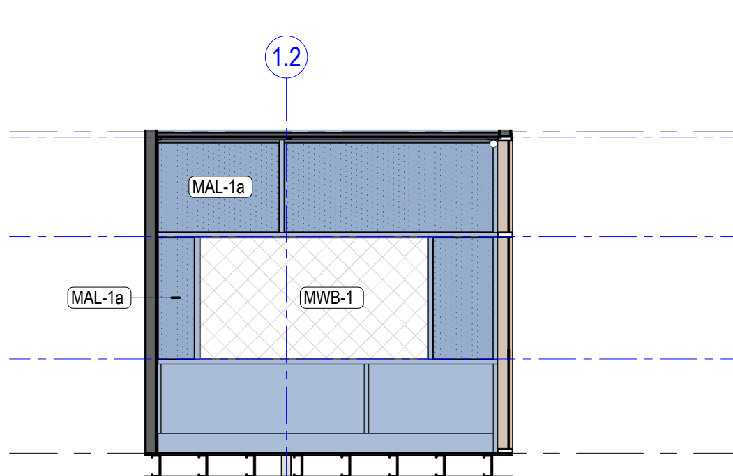
5 0.31 - Meeting 4 - West Elevation 1 : 50
