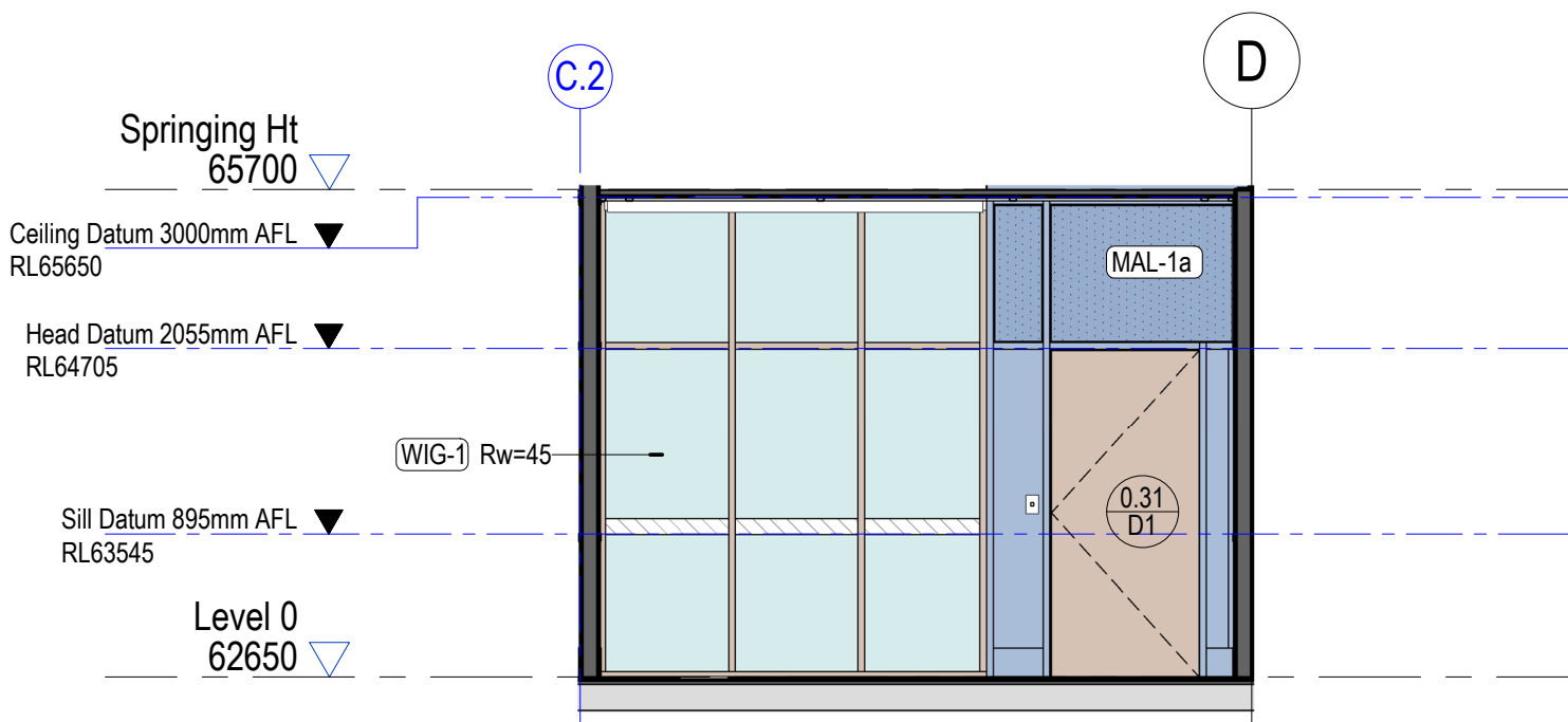
2 0.31 - Meeting 4 - North Elevation 1 : 50
