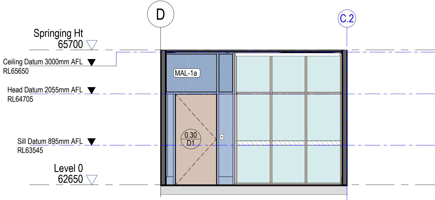
9 0.30 - Meeting 3 - South Elevation 1 : 50
