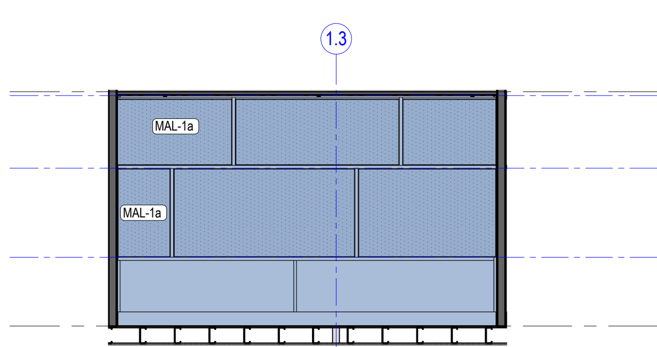
8 0.30 - Meeting 3 - East Elevation 1 : 50
